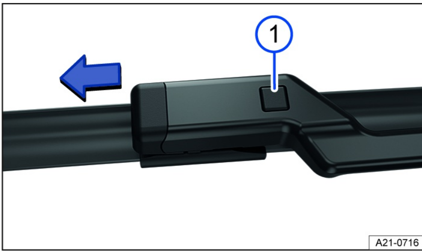
Fig. 142 Changing the windshield wiper blades.
