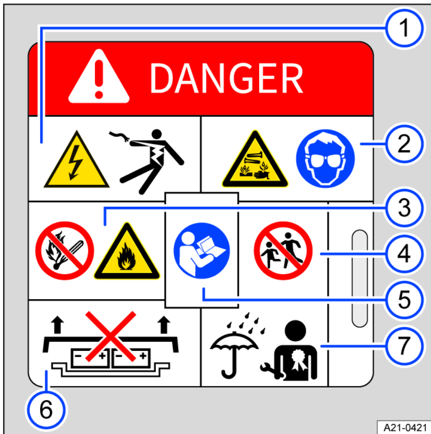
Fig. 128 Warning sign on the high-voltage battery.
