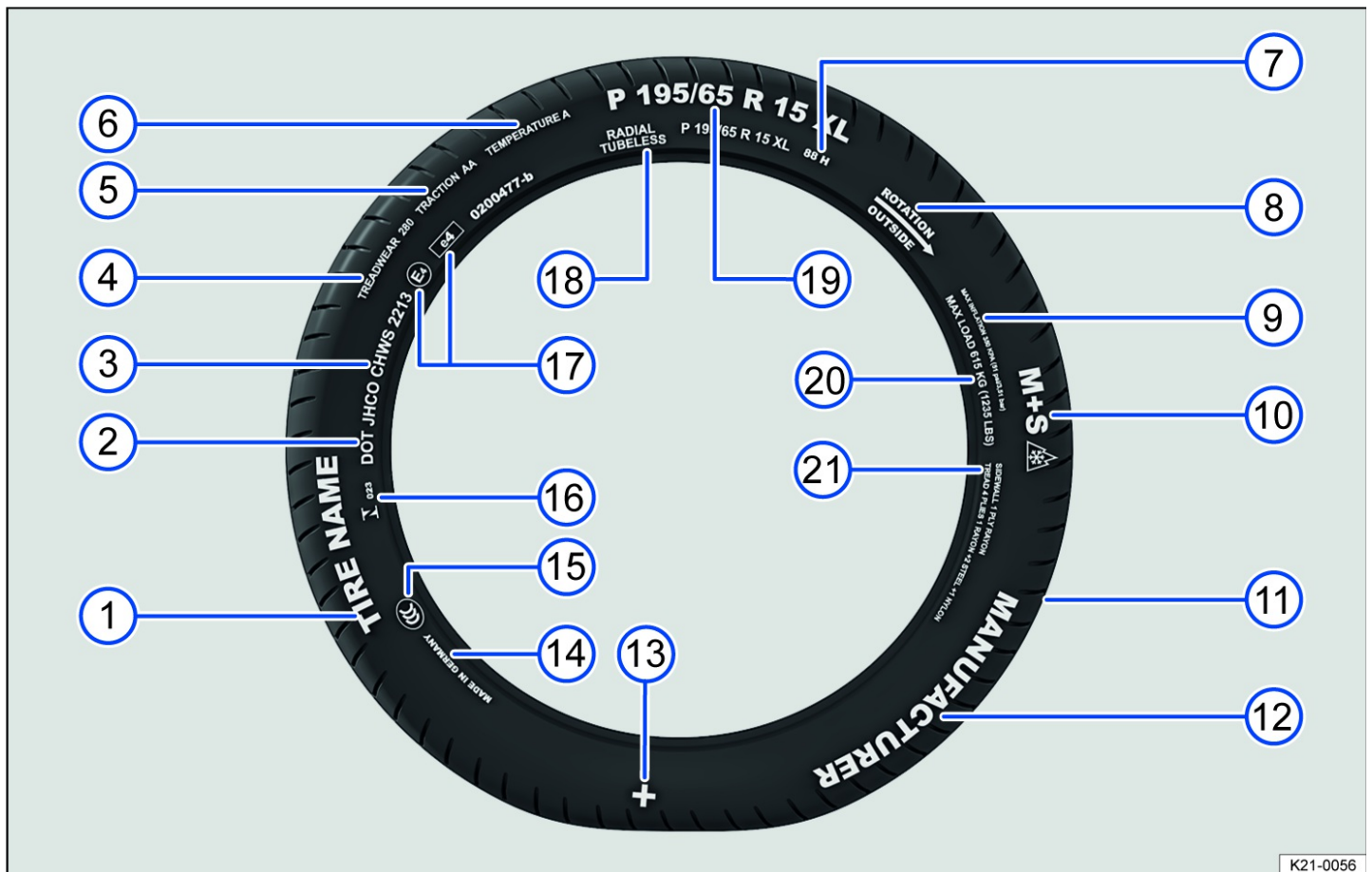
Fig. 177 International tire labeling.
