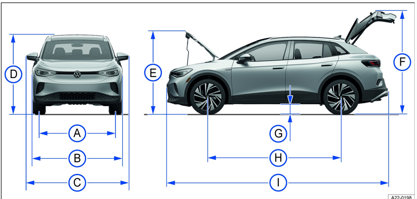
Fig. 187 Vehicle dimensions.
