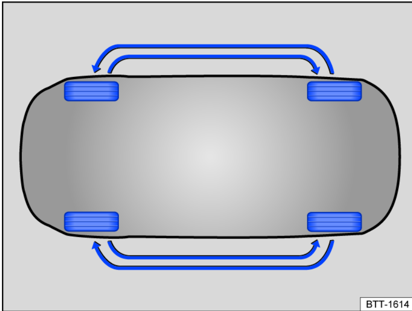
Fig. 165 General example: Diagram for replacing the wheels with the same tire and rim size on all wheels.
