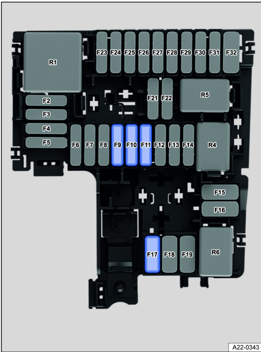
Fig. 146 In the hood space: Fuse locations.
