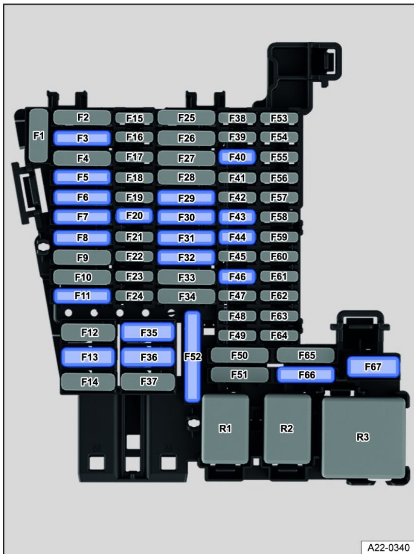
Fig. 149 Fuse assignment in the instrument panel.
