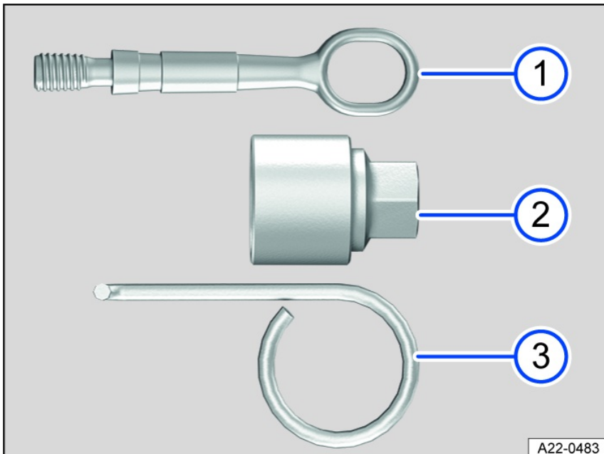
Fig. 138 Vehicle tool kit components (general example).
