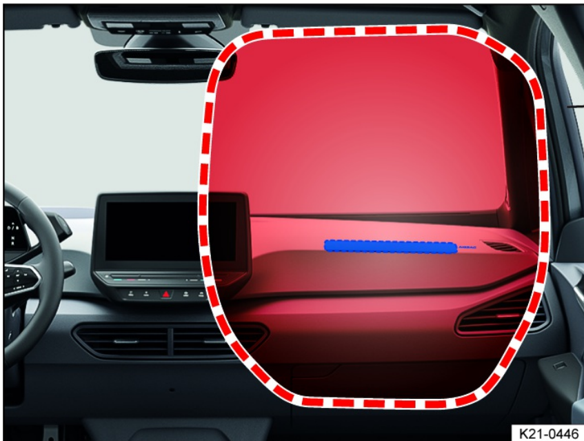
Fig. 24 Installation location and deployment zone of the front passenger's front airbag.
