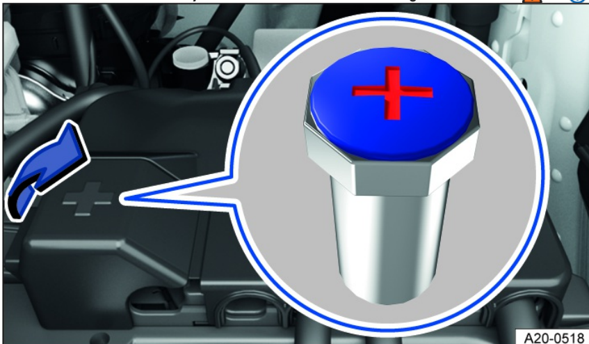
Fig. 153 Under a cover in the hood space: Positive jump-start point.
