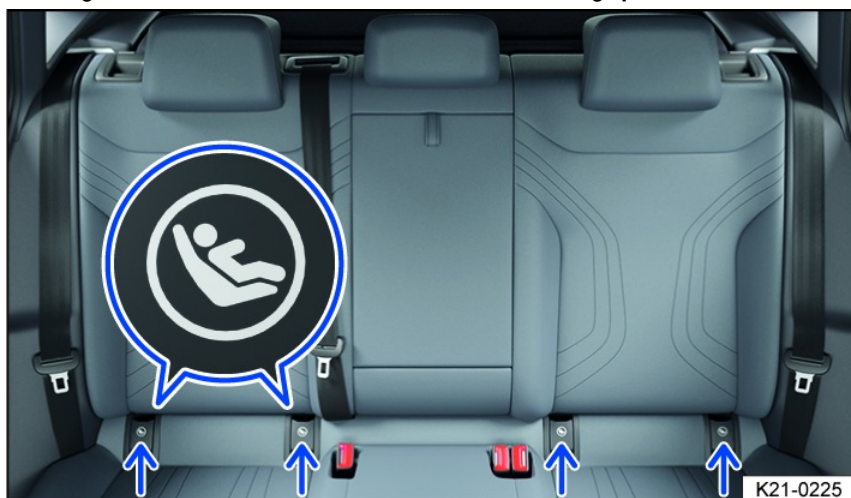
Fig. 29 On the outer seats in the rear bench seat: Designation of the ISOFIX/lower LATCH anchorage points for child restraints.
