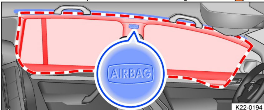
Fig. 27 On the left side of the vehicle: installation location and deployment zone of the Side Curtain Protection®.
