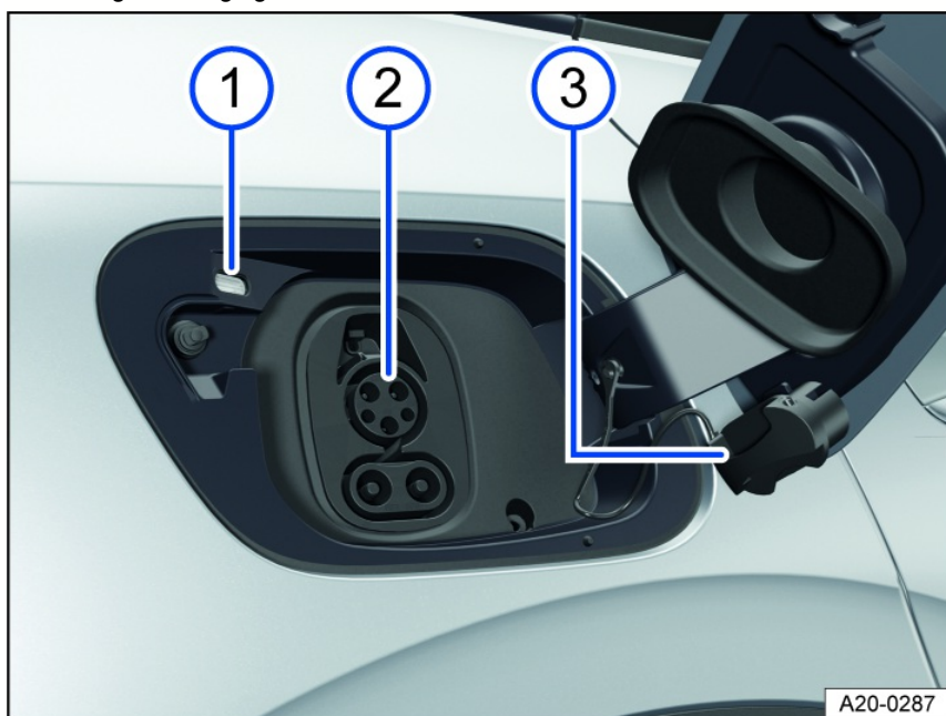
Fig. 129 Behind the rear-right charging socket flap: Charging socket.
